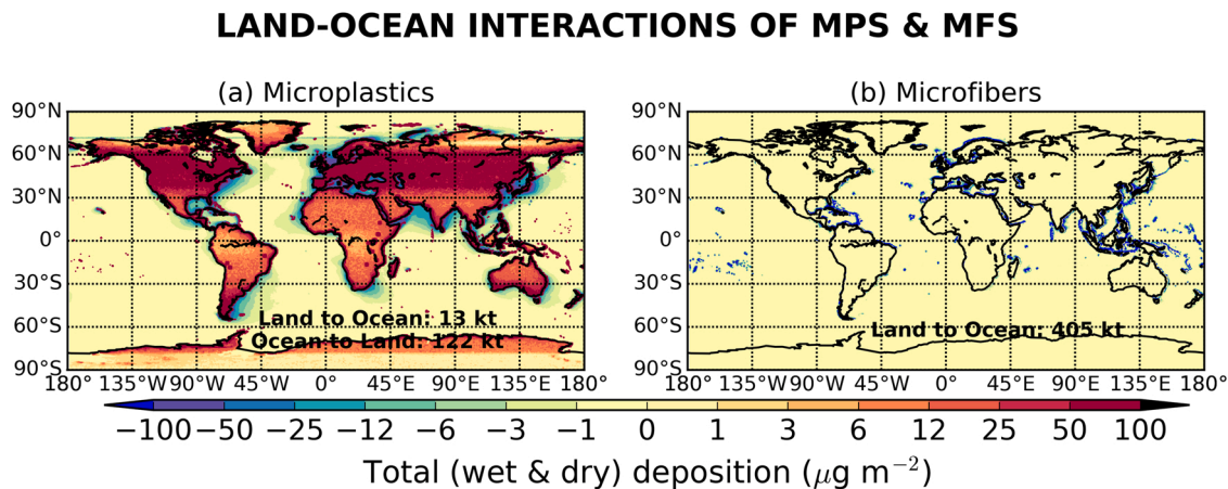
Fig. 7. (a) MPs emitted from the land that were deposited over the ocean annually and vice versa (ocean to land). (b) MFs emitted from global population that were deposited in the ocean.
